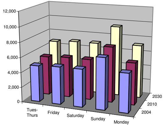
Estimated Daily Traffic Volume on MM Bridge (EB) - June
