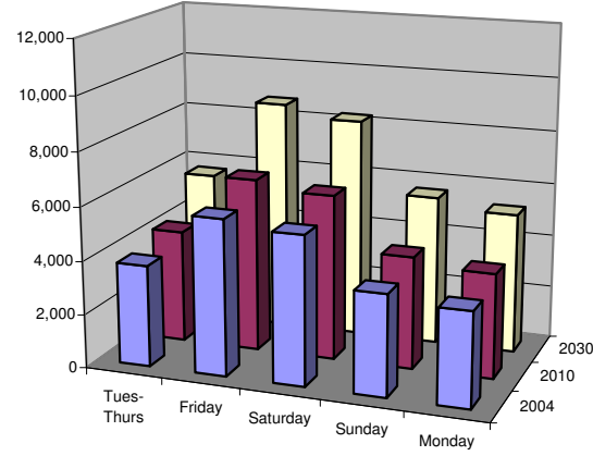
Estimated Daily Traffic Volume on MM Bridge (WB) - July
