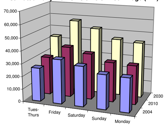
Estimated Daily Traffic Volume on I-80 Bridge (WB) - June
